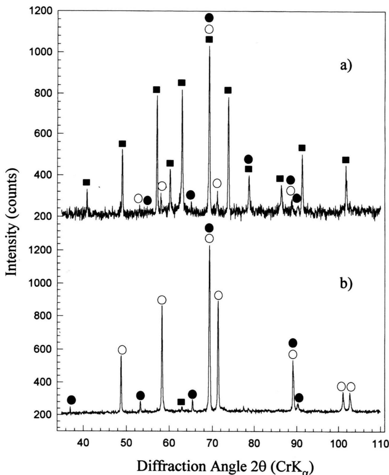
Fig. 2. X-ray diffraction patterns for FeB-CrB powder mixtures treated for 8 h: \text{Cr}/(\text{Cr}+\text{Fe})=0.1 (a) and 0.8 (b) (○) CrB, (■) FeB and (□) \text{Fe}_2\text{B} .
