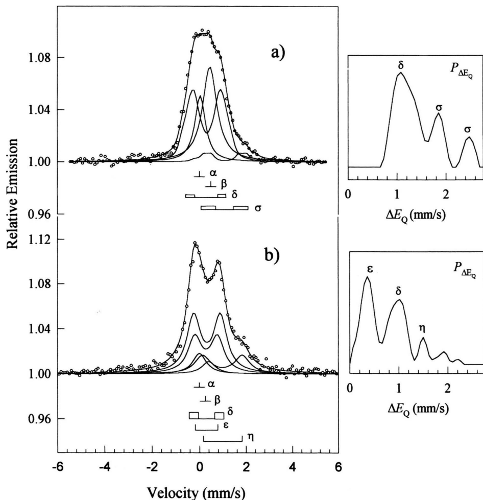
Fig. 6. Conversion electron Mössbauer spectra and quadrupole splitting ( \Delta E_Q ) distributions for 5Fe film (a) and 5Fe/2Al bilayer (b) aged at room temperature in air.
