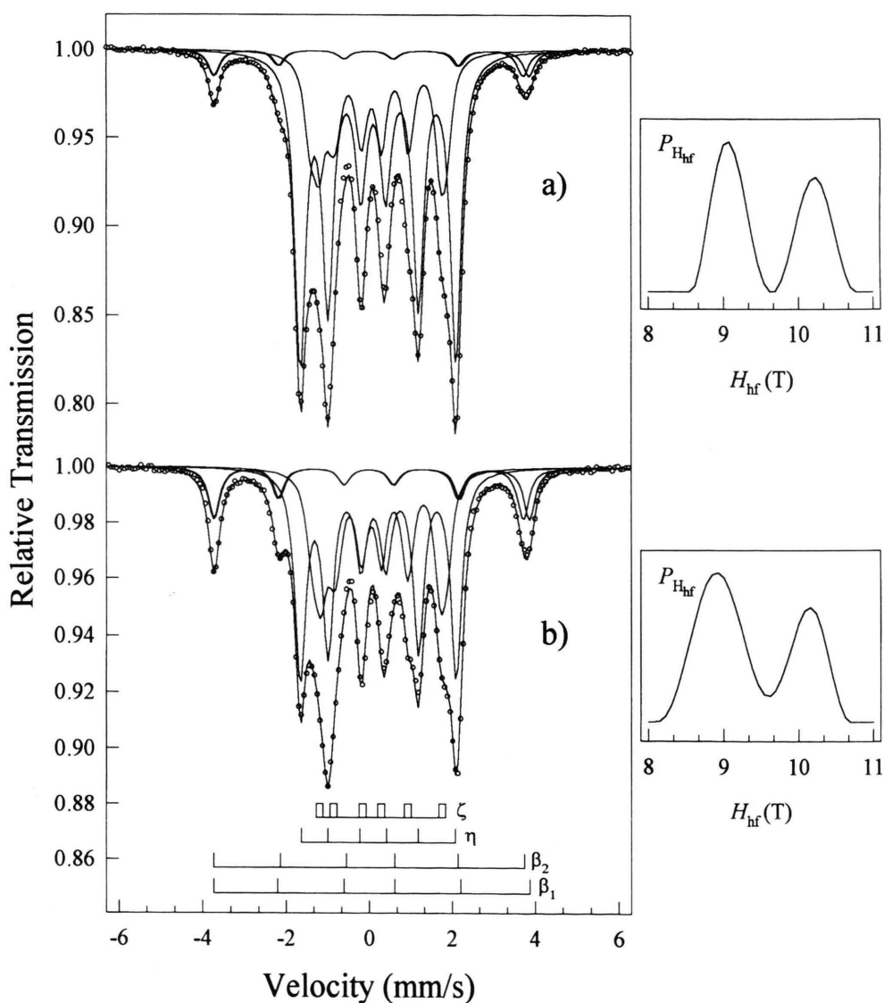
Fig. 1. Mössbauer spectra and hyperfine magnetic field ( H_{\text{hf}} ) distributions of \zeta contribution for FeB-CrB powder mixtures thermally treated for 8 h: \text{Cr}/(\text{Cr} + \text{Fe}) = 0.1 (a) and 0.4 (b).
